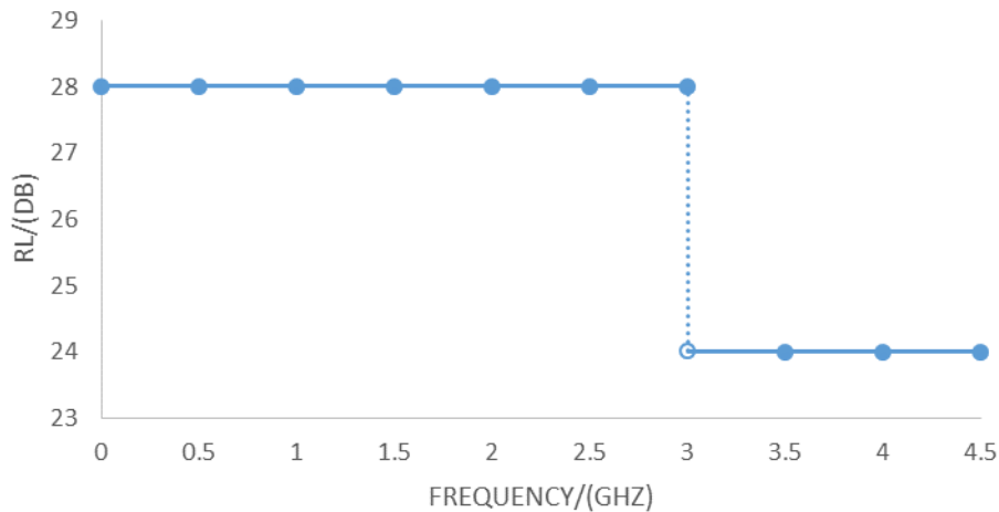
A1505ADHD3 Minimum Return Loss
